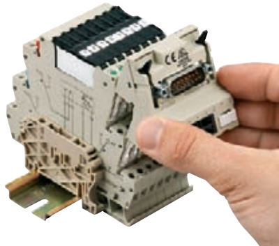
Insert the adapter onto the cross-connection rail and make sure that it is in the correct position
