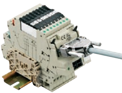
Connect the pre-assembled cable fitted with a HE-10 or SUB-D connector
